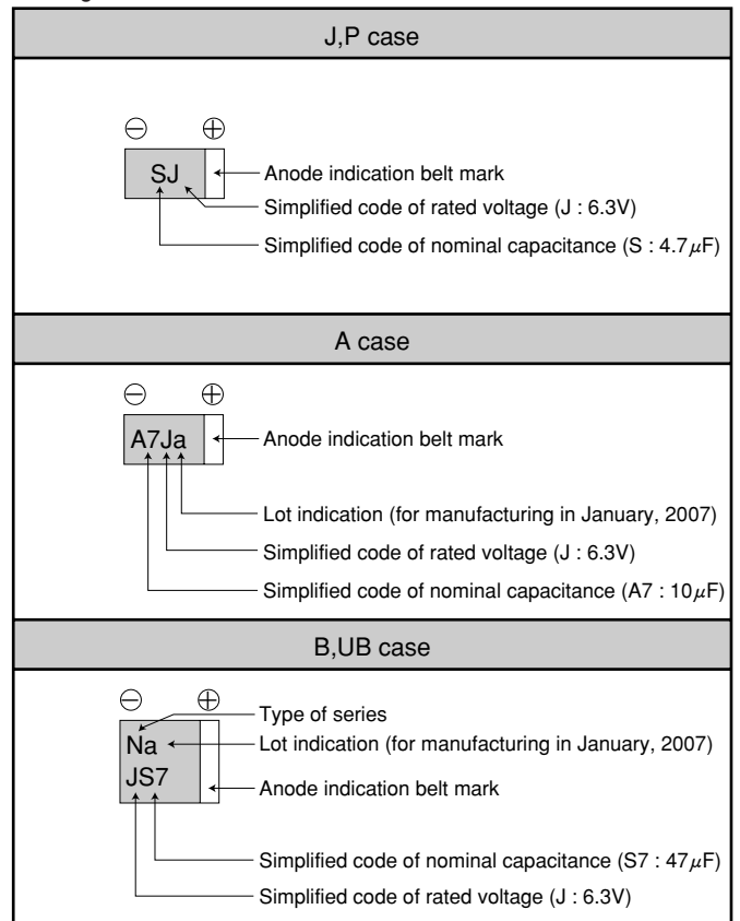
Marking indication TNC series
